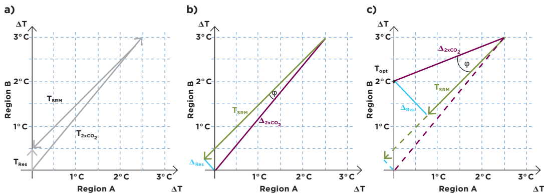
Figure 2 a–c: Graphical representation of the two-region example. The origin represents the baseline temperature configuration. Panel 2a shows the temperature changes in the case of a doubling of \text{CO}_2 with and without a specific SRM intervention designed to restore temperatures in Region A. Panel 2b shows the SRM level that minimises global damages if the rationale is to restore the baseline climate. Panel 2c demonstrates that SRM is less capable of establishing an alternative climate target T_{\text{opt}} .
