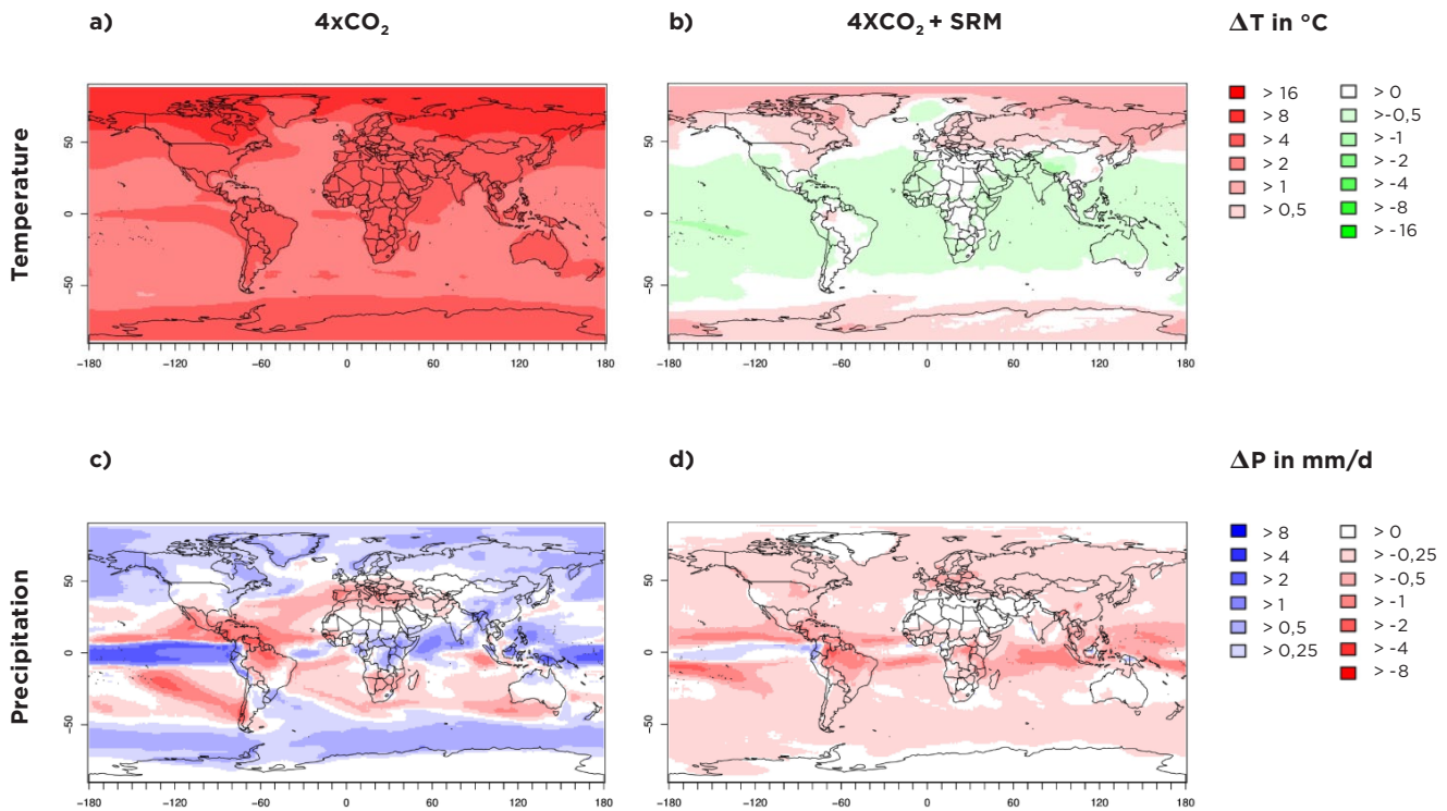
Figure 1: GeoMIP modelling results (Kravitz et al. 2011, 2013) for temperature (top panels) and precipitation (bottom panels) responses to 4\times\text{CO}_2 (left panels) and additional SRM (right panels).
