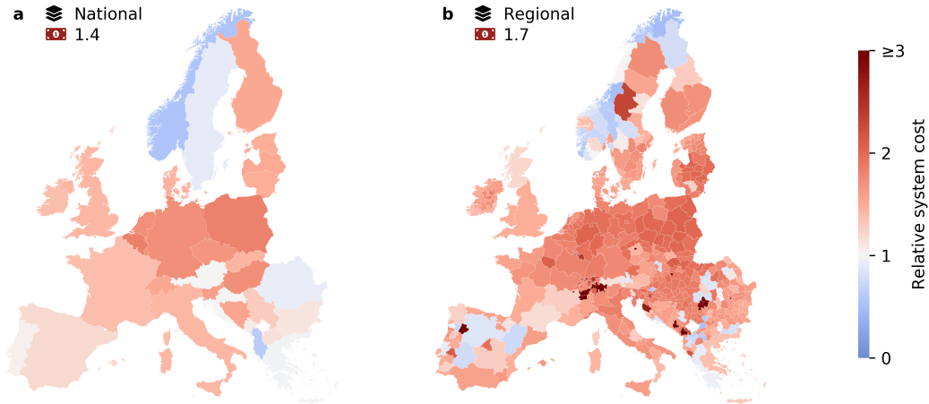
Figure 3.6: Spatial distribution of system cost normalised by demand for entirely national- and regional-scale systems, relative to the European average of the least-cost, entirely continental-scale case. Each panel shows the Europe-wide relative system cost beneath the panel heading. a , Relative system cost for each country in the entirely national-scale system without any exchange of electricity between countries. b , Relative system cost for each region in the entirely regional-scale system without any exchange of electricity between regions.
