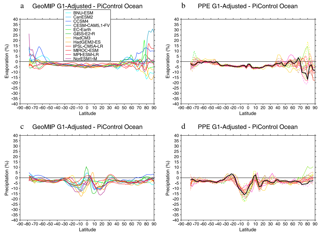
Figure 3. G1-adjusted-piControl zonal, ocean mean of evaporation and precipitation change for the individual members of the (a and c) GeoMIP MME and (b and d) PPE, respectively. The solid black line shows the standard HadCM3 model. Means are calculated from years 11 to 50 of the simulations.
