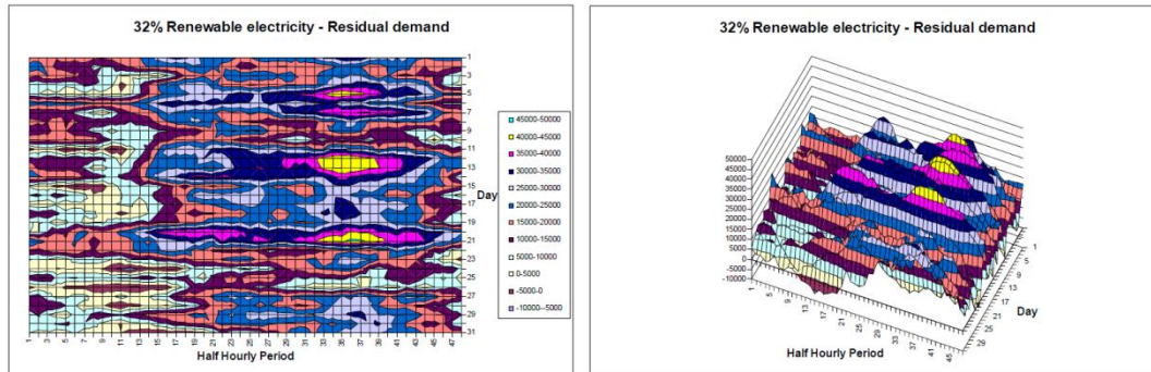
Figure 8: EDF's charts showing the same basic conflict between fluctuating wind and solar as in Figure 4, though the conflict is harder to see. The 3D rendition on the right is clearer but perhaps still too complex for civil society actors hoping to engage with the public. Source: Electricité de France . Public domain, study from 2008.
