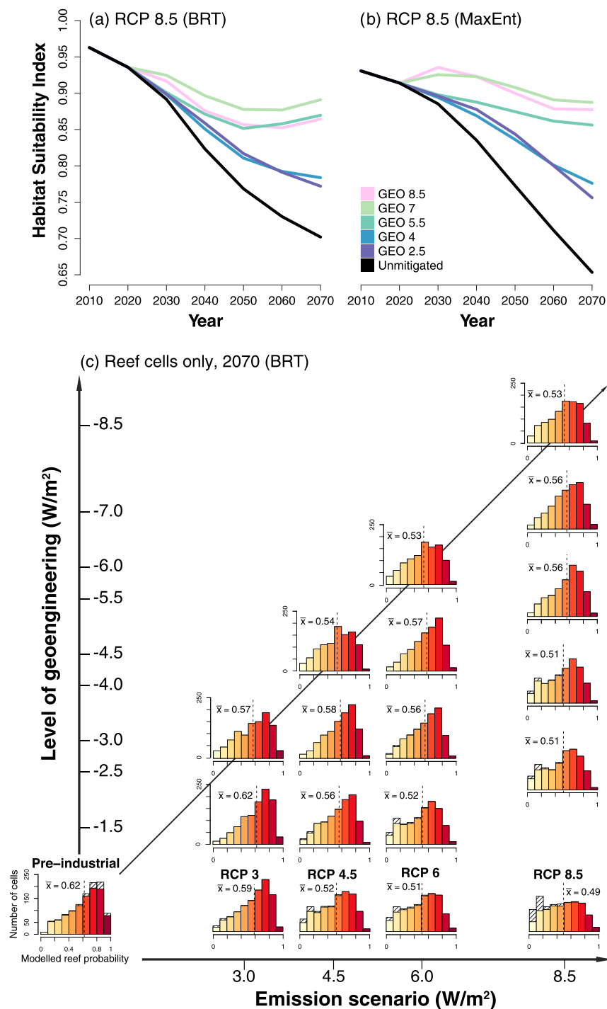
Figure 2. Habitat Suitability Index (defined as the average suitability for coral reefs within the shallow water mask between 60^{\circ}S and 60^{\circ}N ) for (a) BRT and (b) MaxEnt. Values are normalized to preindustrial (P-I) predictions and show the evolution at 10 year intervals until 2070 under the unmitigated RCP 8.5 scenario (black) and various level of SRM (lighter colors show progressively higher degrees of SRM intervention). For all other scenarios, see Appendix S2 and Figures S2.8 and S2.9. (c) Histograms showing the proportion of reef cells within binned BRT modeled suitability values. The bottom left histogram is for P-I conditions; all remaining histograms are for 2070 conditions and reflect potential changes in suitability under the four unmitigated RCPs (bottom row, along x axis) and various levels of SRM geoengineering ( y axis). Reef cells are cells where reefs or non-reef coral communities are presently found (ReefBase v2000). Novel environmental conditions, compared to the 1990 values used for model training, are simulated by UVic Earth System Climate Model for SST and \Omega_{Arag} on some reef cells. The solid colored histogram bars contain all cells either with environmental conditions within the bioclimatic envelope used to train the models or where out-of-range variables do not significantly affect predictions. The average suitability value ( \bar{x} ) of reef cells for each scenario is calculated from this sample set. Cells where predictions are less reliable (i.e., SST and/or \Omega_{Arag} values out of training range and MaxEnt clamping value > 0.1 ; see Appendix S3) are indicated by hatched pattern and have been excluded from the calculated average.
