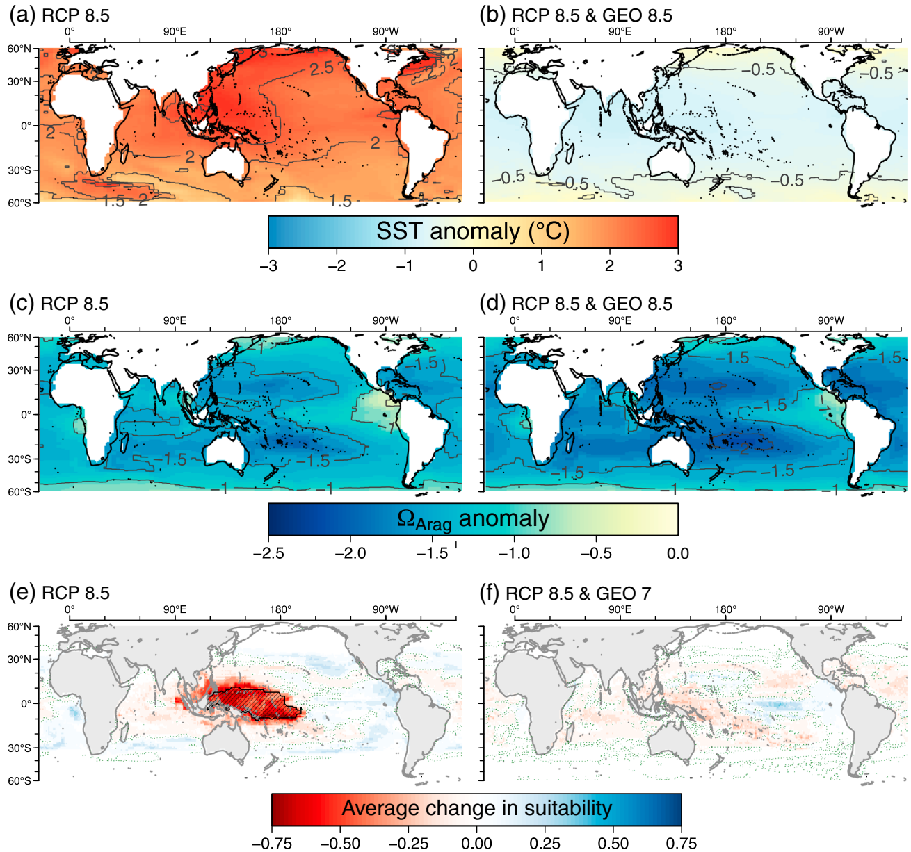
Figure 1. Simulated spatial anomalies, year 2070 minus preindustrial (P-I), of (top, a and b) sea surface temperature (SST) and (bottom, c and d) aragonite saturation state ( \Omega_{Arag} ) under RCP 8.5 (a and c) and with SRM geoengineering returning total anthropogenic radiative forcing to P-I values in the “RCP 8.5 & GEO 8.5” scenario (b and d). Change in shallow water tropical coral reef habitat suitability between 2070 and P-I, averaged from BRT and MaxEnt model outputs for RCP 8.5 (e) and “RCP 8.5 & GEO 7,” with SRM geoengineering to reduce anthropogenic radiative forcing to 1.5 \text{ W/m}^2 above P-I by 2100 (f). Green dotted line corresponds to 0 change; black hatched pattern overlays area where projections move beyond training range with significant influence on predictions. For other scenarios, see Appendix S2.
