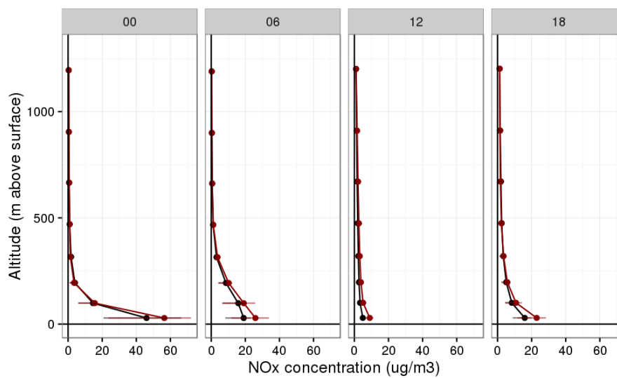
Figure S10. The figure shows mean \text{NO}_x profiles in the lower troposphere simulated with a 1\text{km}\times 1\text{km} model resolution at 00:00, 06:00, 12:00 and 18:00 UTC, for the base run (black) and S3 (downscaled emissions, red), for Amrumer Straße. Error bars give the 25th and 75th percentiles.
